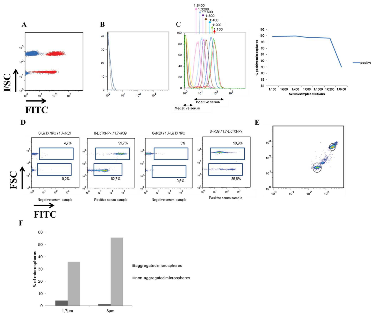
Figure 1. Optimization of the experimental conditions. (A) Unspecific binding of serum antibodies to uncoated magnetic microspheres. Positive serum sample is represented in red, while negative serum sample in blue. (B) BfS as blocking agents (blue for positive serum and black for negative). (C) Positive and negative serum samples diluted from 1:100 to 1:6400. (D) PMSI-8.07Ni-NTA coated with rK39 and PMSI-1.7Ni-NTA coated with LicTXNPx in the presence of a positive serum or a negative serum and PMSI-8.07Ni-NTA coated with LicTXNPx and PMSI-1.7Ni-NTA coated with rK39 in the presence of a positive serum or a negative serum. (E) PMSI-8.07Ni-NTA coated with rK39 and PMSI-1.7Ni-NTA coated with LicTXNPx formed populations of different sizes as consequence of microspheres aggregation. For further analysis, only the non-aggregated populations (black line) were used. (F) Percentage of aggregated microspheres is higher in PMSI-1.7Ni-NTA than in PMSI-8.07Ni-NTA microspheres. doi:10.1371/journal.pntd.0002371.g001
