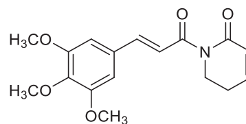
Fig. 1 Chemical structure of pipartine
